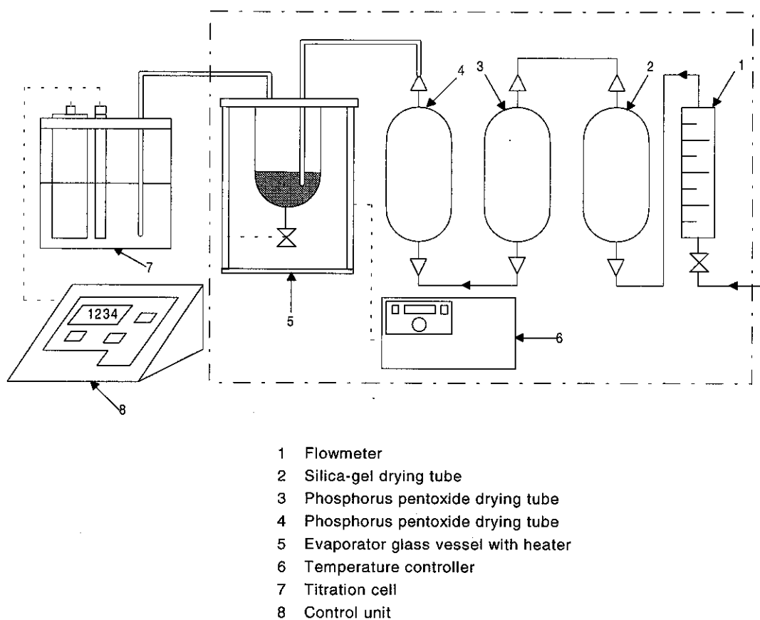
Figure 3 – Block diagram of automatic titrator and evaporation stripping unit
